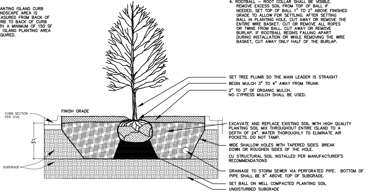
○ TREE PLANTING IN A PARKING LOT ISLAND NOT TO SCALE
