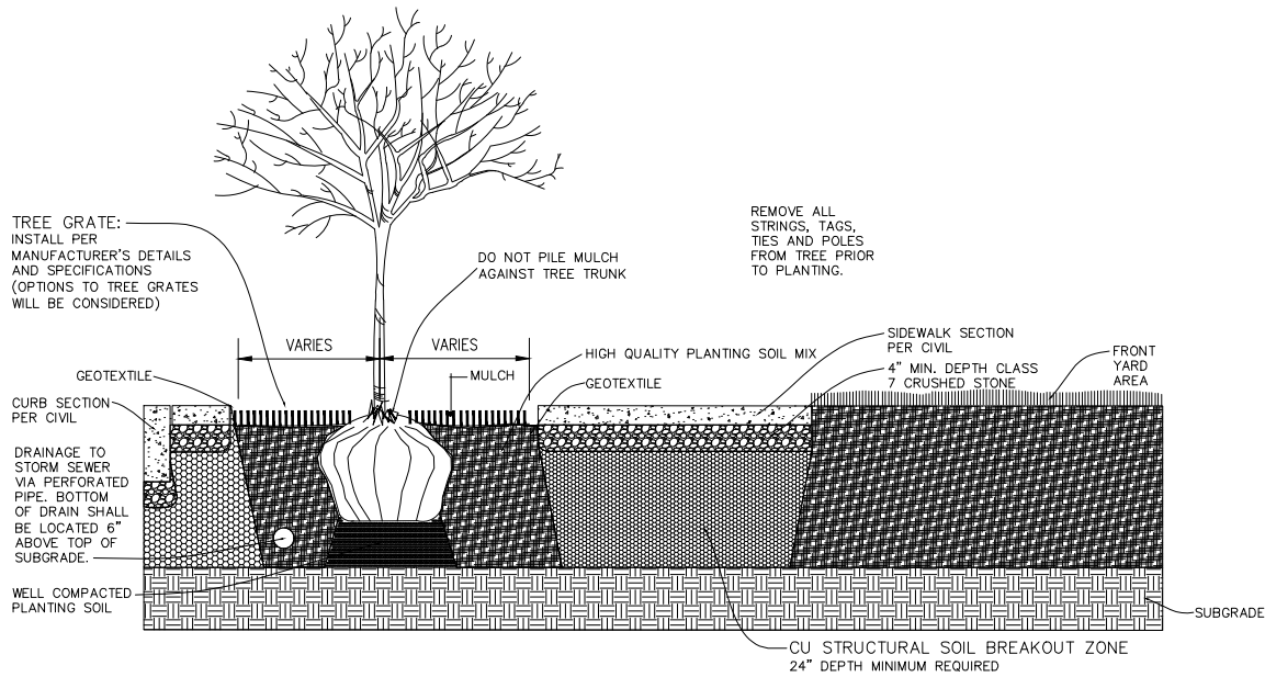
STRUCTURAL SOIL BREAKOUT ZONE FROM NARROW TREE LAWN TO FRONT YARD DETAIL
